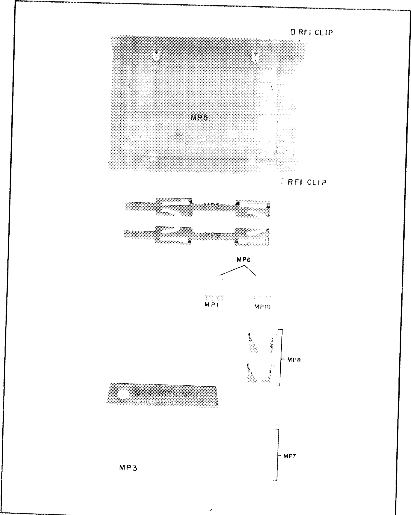
Figure 6-1. 5300B Mainframe Mechanical Parts
