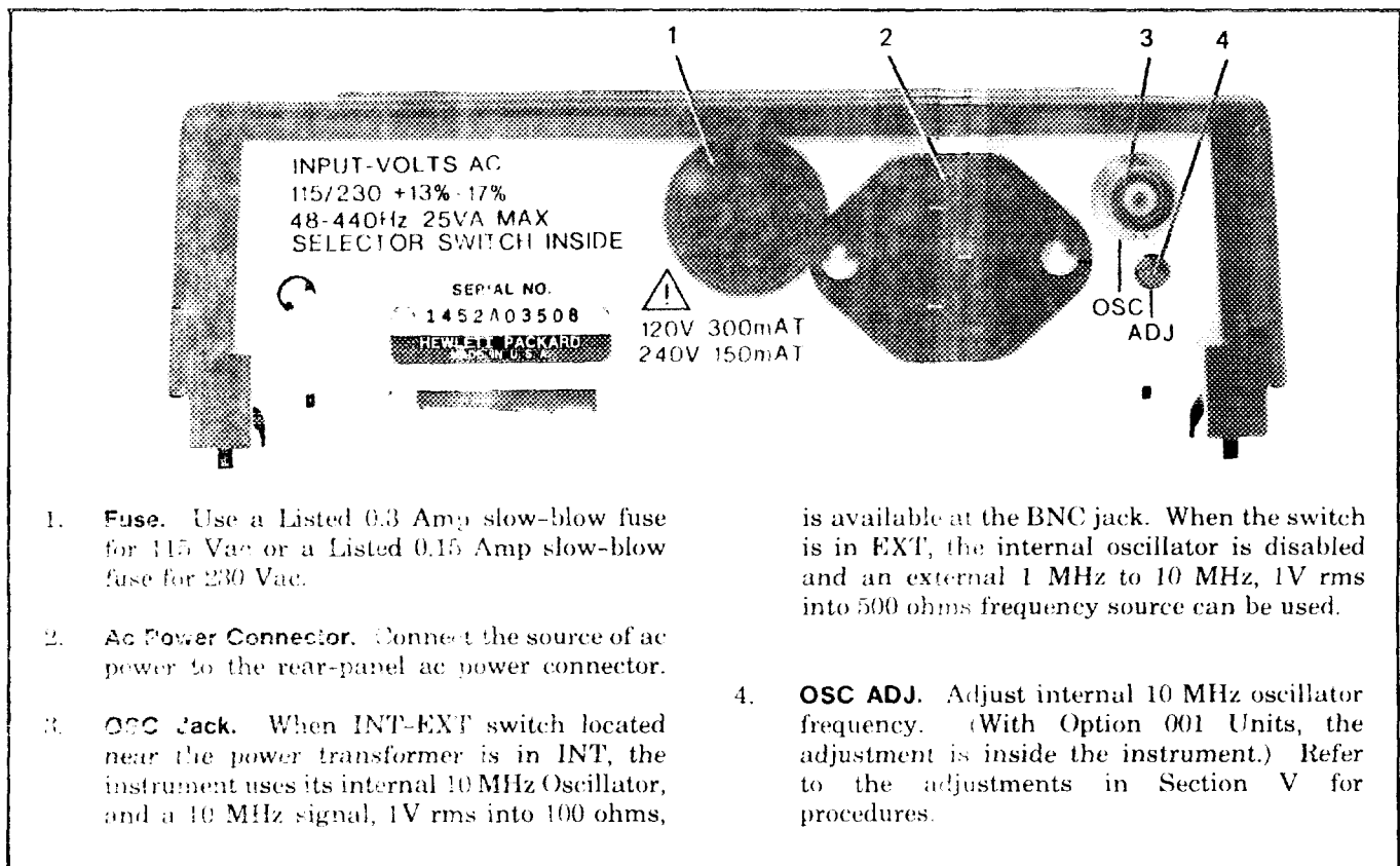
Figure 3-2. Rear Panel Connectors
