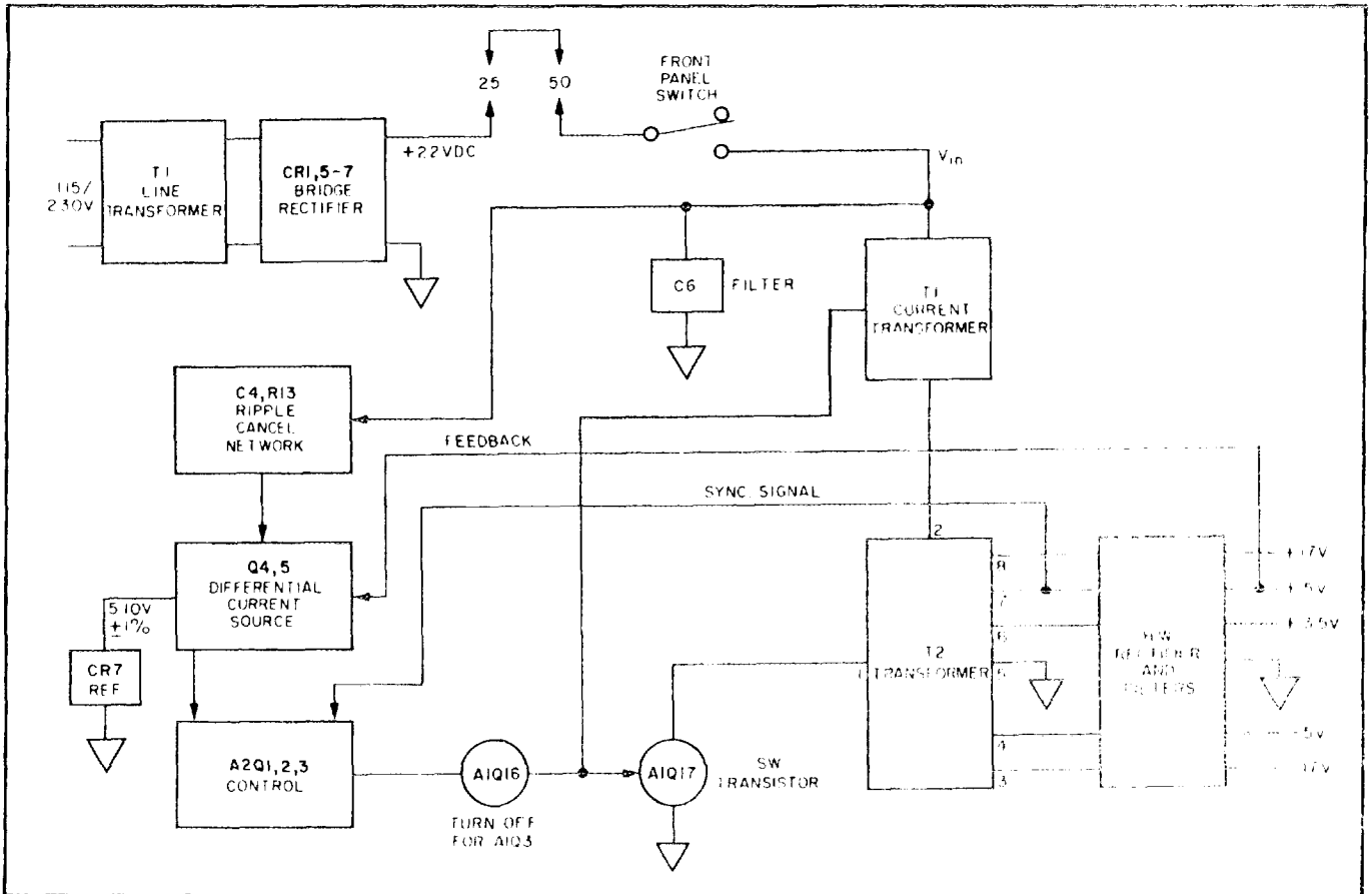
Figure 4-5. Power Supply Block Diagram
