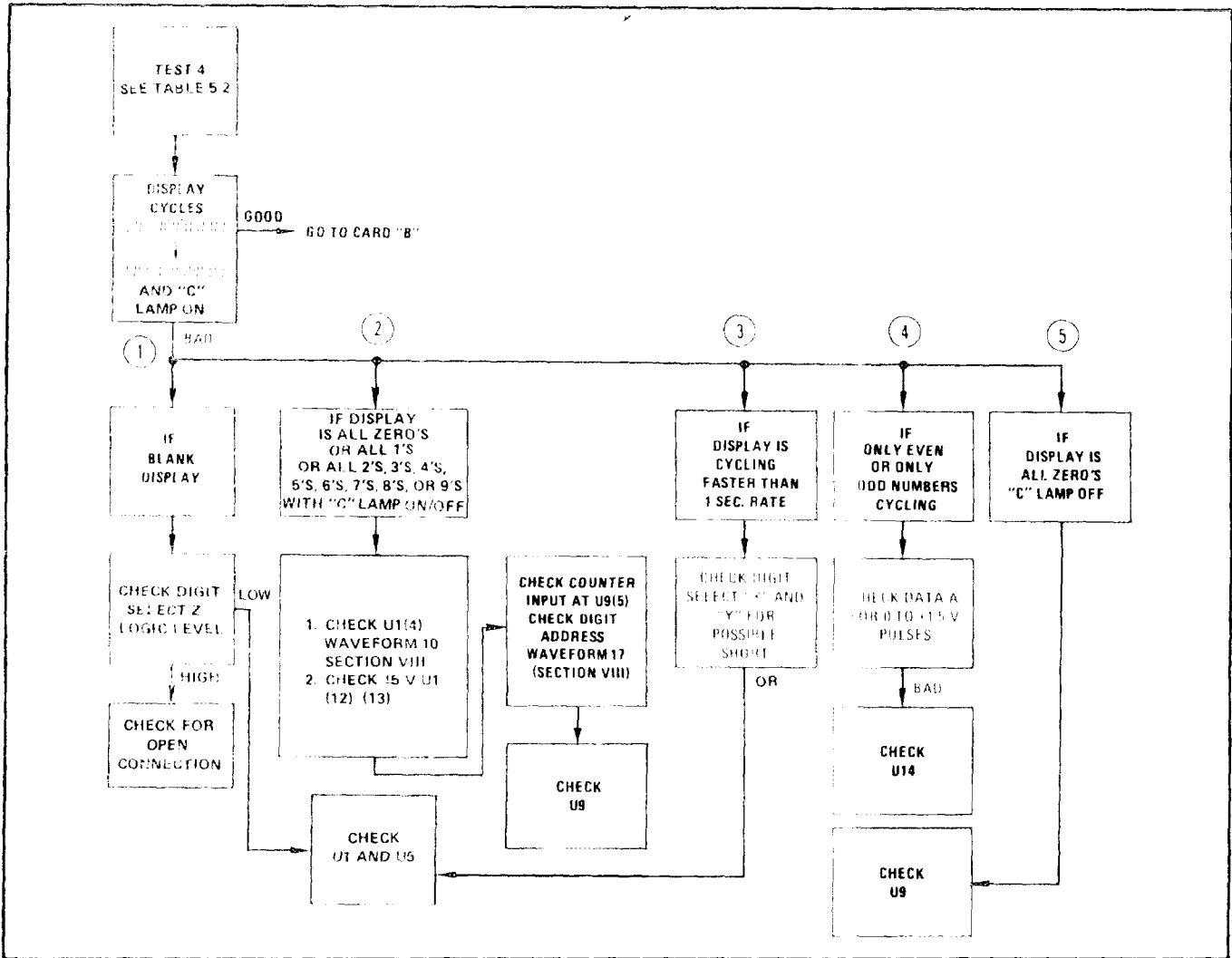
Figure 5-4. Display Checks
